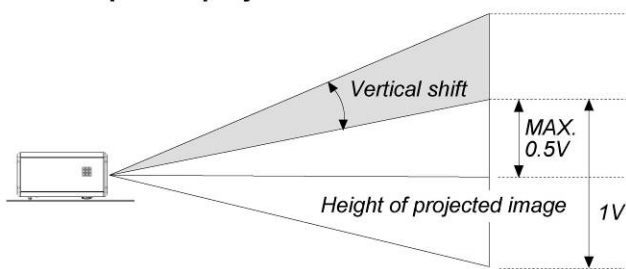
Desktop front projection
