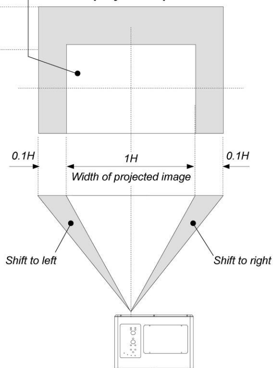
Normal projection position
